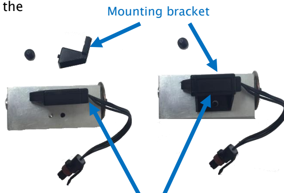
1711526 "A/C Clutch Cycle Switch" / "Refrigerant Flow Sensor"
