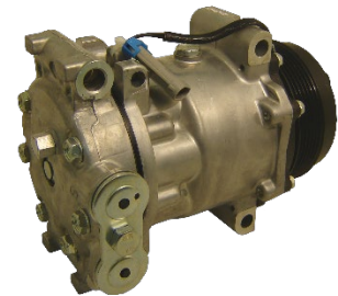
gpd compressor 6512124 is a Sanden style replacement for 6511338
