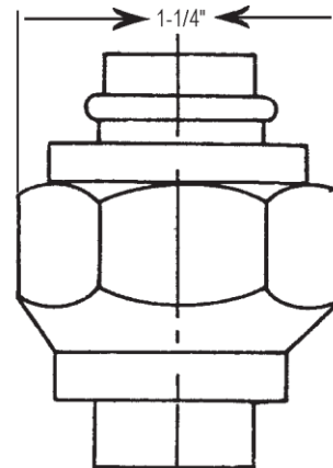
No. 12 1 - 1/16" - 14 Thread
