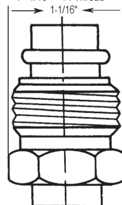
No. 12 1 - 1/16" - 16 Thread
