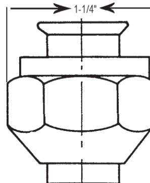
No. 12 1 - 1/16" - 14 Thread
